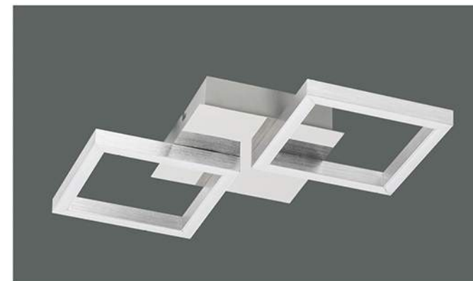
C3433201BA 32W 2560lm 3000K 230V~50Hz Brush/Metal+Plastic 750x370x60mm
