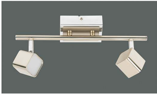
S2401401NK 8W 640lm 3000K 230V~50Hz Nickel/Metal+Plastic
