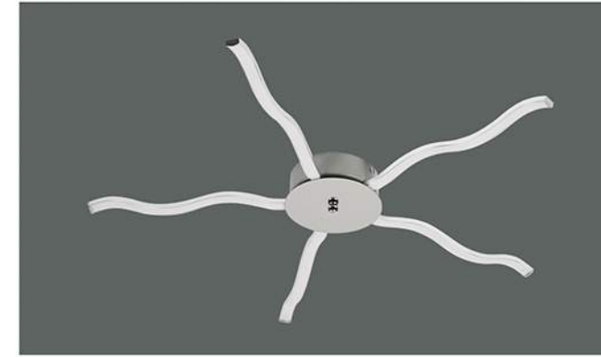
C3542002BR 20W 1600lm 3000K 230V~50Hz Chrome/Metal+Plastic
