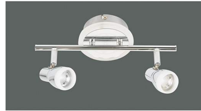
S2241001BR 8+2W 700lm 3000K 230V~50Hz Chrome/Metal+Plastic
