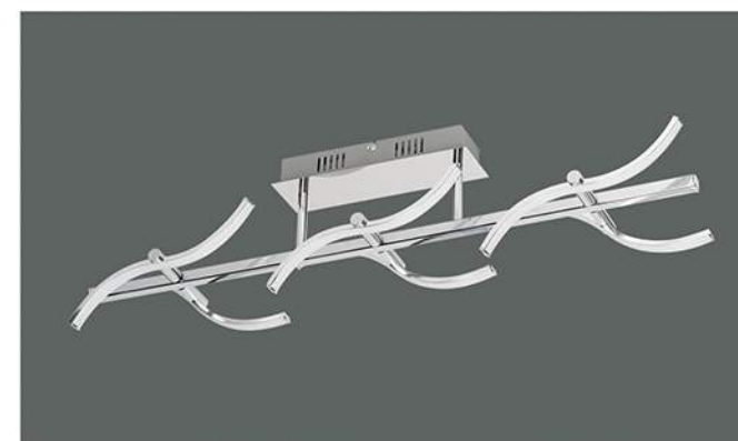
C3520624BR 24W 1920lm 3000K 230V~50Hz Chrome/Metal+Plastic 780x130x160mm
